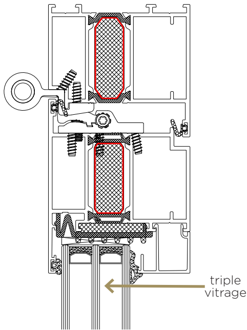
Version 1 Triple vitrage
